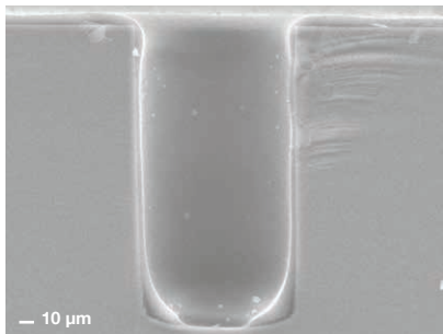
Bottom opening of a coated TSV combining Spray Coated 90° deep VIA exposure on EVG® IQ Aligner NT® Source: EVG
