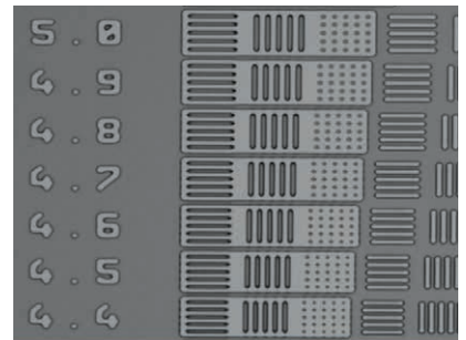
1 μm thick resist with a resolution below 5 μm with a large proximity gap of 30 μm exposed on EVG® IQ Aligner NT®, Source: EVG
