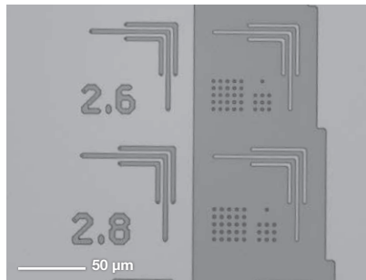
1 μm thick resist with 2.6 μm resolution exposed on EVG®620 NT in 15 μm proximity Source: EVG
