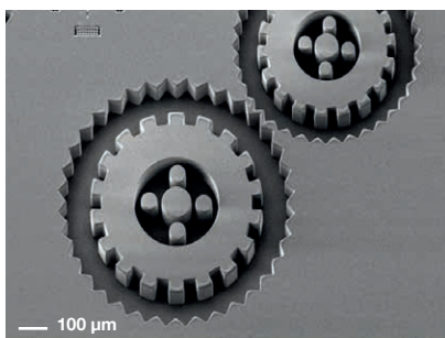
High aspect ratio structures for LIGA structures with a 200 μm thick resist exposed on EVG®6200 NT Source: EVG
