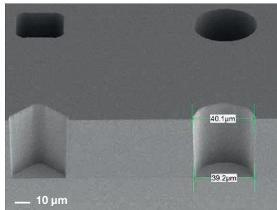
Bumping results in a 40 μm thick resist performed on EVG® IQ Aligner NT® Source: EVG
